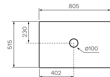
PORCELAIN TOP VIEW
